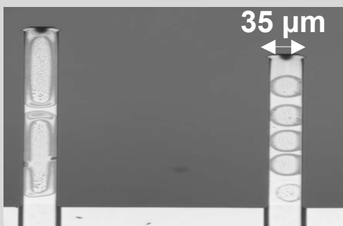
Drops as small as 35 \mu\text{m} can be placed on individual cantilevers
